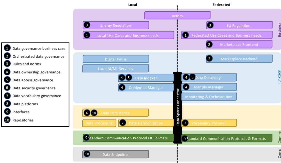
Figure 3. DERA 3.0 link to data governance
