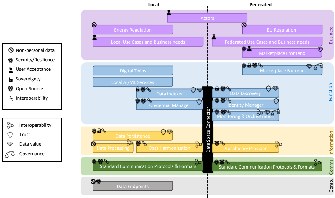
Figure 2. DERA 3.0 layered architecture and link to the DESAP and OpenDEI building blocks.
